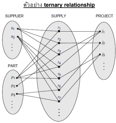
Figure 7.10 Some relationship instances in the SUPPLY ternary relationship set.
