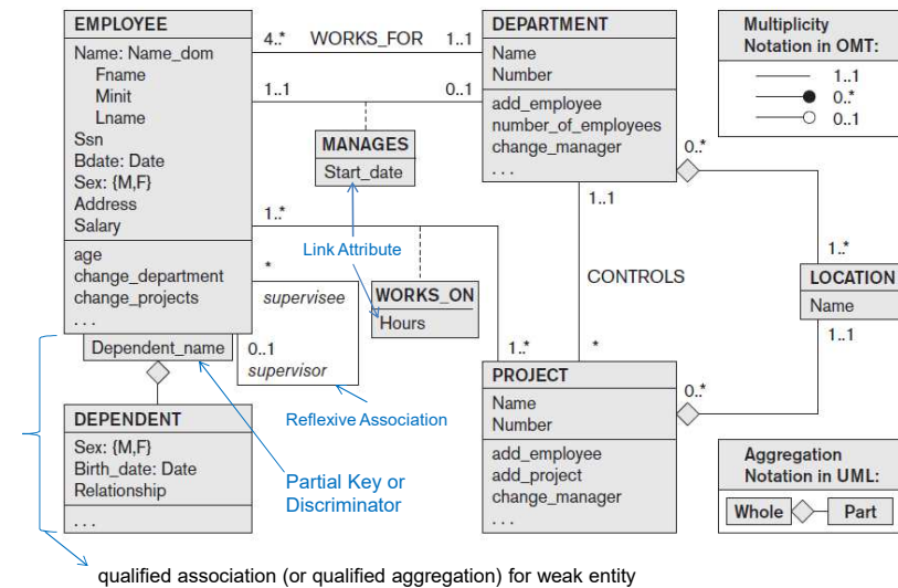
Figure 7.16 The COMPANY conceptual schema in UML class diagram notation.
